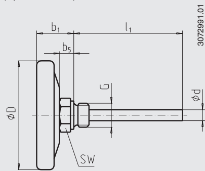
Back mount (BM) (up to 250 °C)
