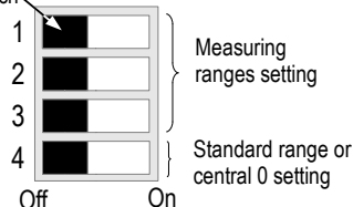
On-off switch Left DIP switch
